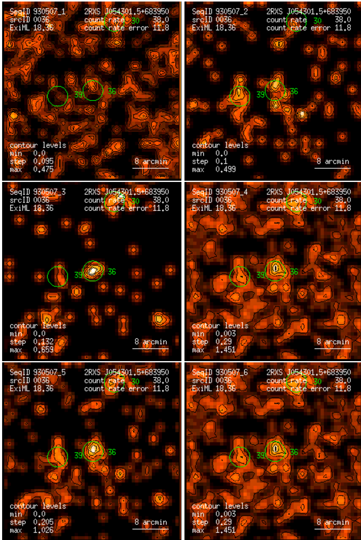
Figure 36: RASS 930507: detection 0036: band rate images, Gaussian filter: (1) PSPC channels 11 – 41, (2) 52 – 90, (3) 91 – 201, (4) 11 – 235, (5) 52 – 201, (6) 11 – 201. Broad band rates in counts/ks. Band rate contour levels in counts/ks/arcmin 2 .
