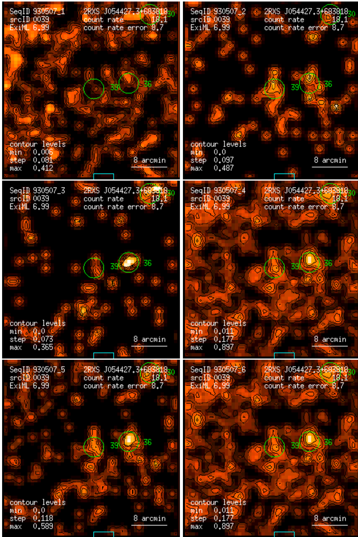
Figure 39: RASS 930507: detection 0039: band rate images, Gaussian filter: (1) PSPC channels 11 – 41, (2) 52 – 90, (3) 91 – 201, (4) 11 – 235, (5) 52 – 201, (6) 11 – 201. Broad band rates in counts/ks. Band rate contour levels in counts/ks/arcmin 2 .
