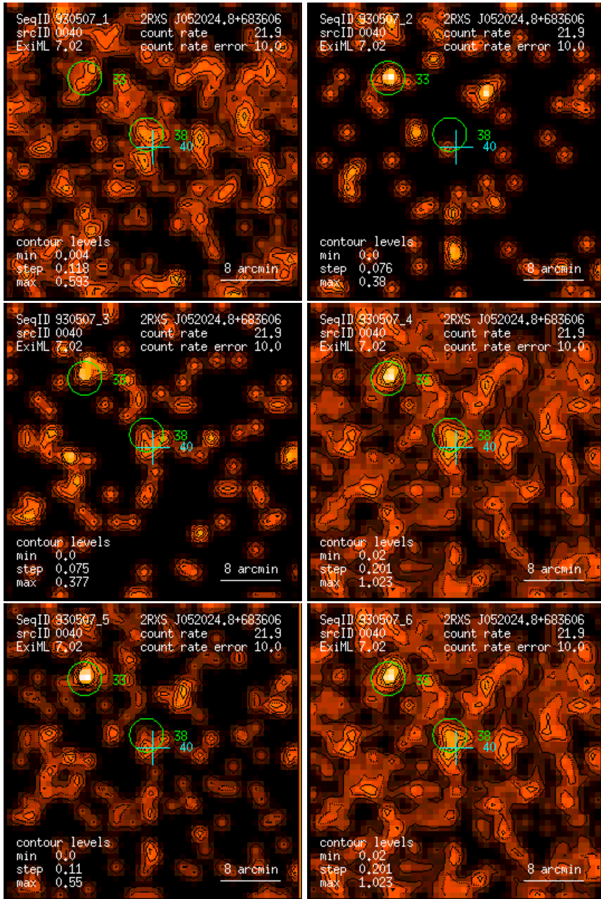
Figure 40: RASS 930507: detection 0040: band rate images, Gaussian filter: (1) PSPC channels 11 – 41, (2) 52 – 90, (3) 91 – 201, (4) 11 – 235, (5) 52 – 201, (6) 11 – 201. Broad band rates in counts/ks. Band rate contour levels in counts/ks/arcmin 2 .
