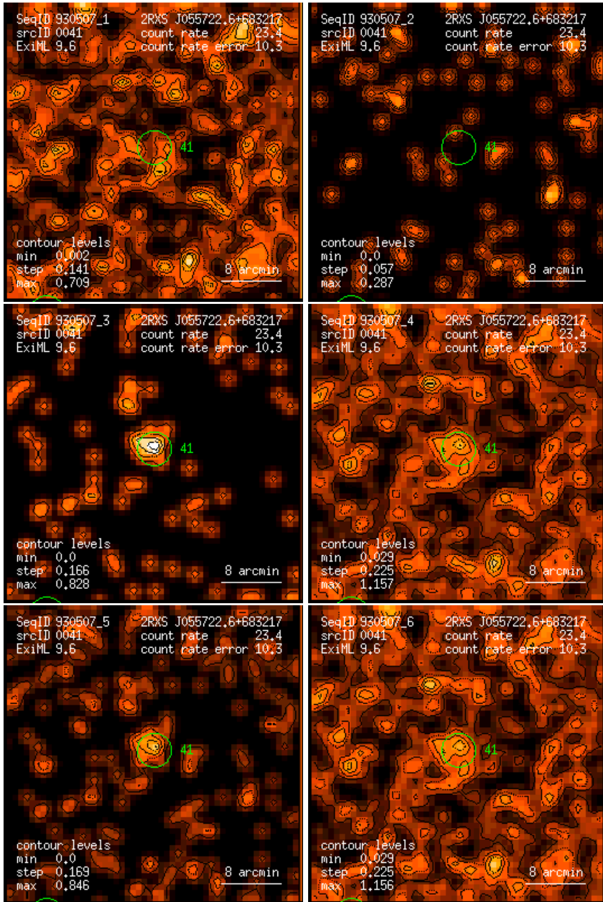
Figure 41: RASS 930507: detection 0041: band rate images, Gaussian filter: (1) PSPC channels 11 – 41, (2) 52 – 90, (3) 91 – 201, (4) 11 – 235, (5) 52 – 201, (6) 11 – 201. Broad band rates in counts/ks. Band rate contour levels in counts/ks/arcmin 2 .
