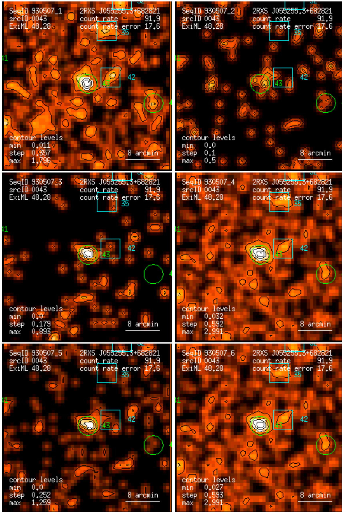
Figure 43: RASS 930507: detection 0043: band rate images, Gaussian filter: (1) PSPC channels 11 – 41, (2) 52 – 90, (3) 91 – 201, (4) 11 – 235, (5) 52 – 201, (6) 11 – 201. Broad band rates in counts/ks. Band rate contour levels in counts/ks/arcmin 2 .
