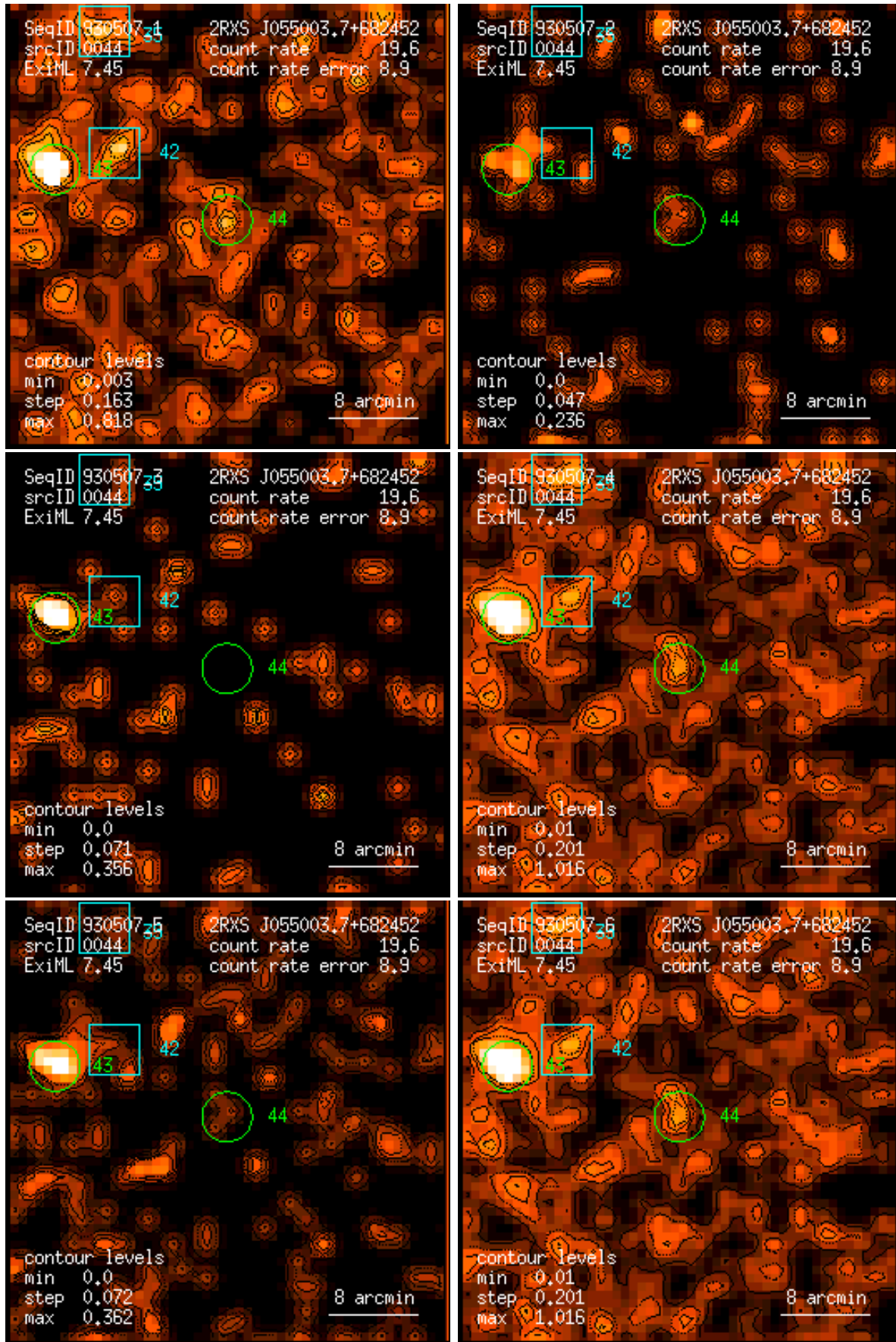
Figure 44: RASS 930507: detection 0044: band rate images, Gaussian filter: (1) PSPC channels 11 – 41, (2) 52 – 90, (3) 91 – 201, (4) 11 – 235, (5) 52 – 201, (6) 11 – 201. Broad band rates in counts/ks. Band rate contour levels in counts/ks/arcmin 2 .
