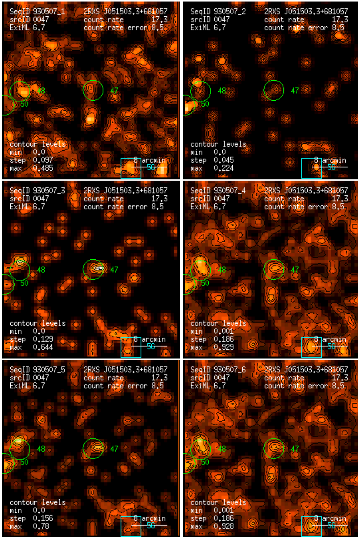
Figure 47: RASS 930507: detection 0047: band rate images, Gaussian filter: (1) PSPC channels 11 – 41, (2) 52 – 90, (3) 91 – 201, (4) 11 – 235, (5) 52 – 201, (6) 11 – 201. Broad band rates in counts/ks. Band rate contour levels in counts/ks/arcmin 2 .
