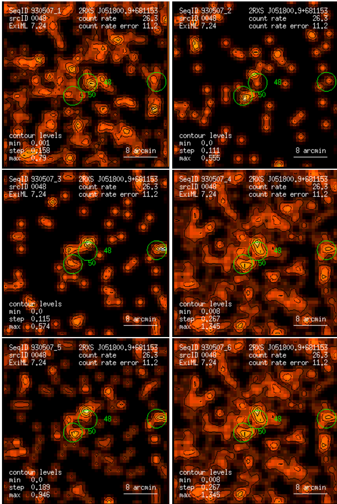
Figure 48: RASS 930507: detection 0048: band rate images, Gaussian filter: (1) PSPC channels 11 – 41, (2) 52 – 90, (3) 91 – 201, (4) 11 – 235, (5) 52 – 201, (6) 11 – 201. Broad band rates in counts/ks. Band rate contour levels in counts/ks/arcmin 2 .
