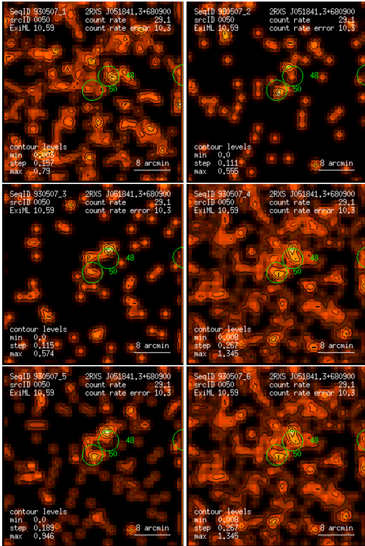
Figure 50: RASS 930507: detection 0050: band rate images, Gaussian filter: (1) PSPC channels 11 – 41, (2) 52 – 90, (3) 91 – 201, (4) 11 – 235, (5) 52 – 201, (6) 11 – 201. Broad band rates in counts/ks. Band rate contour levels in counts/ks/arcmin 2 .
