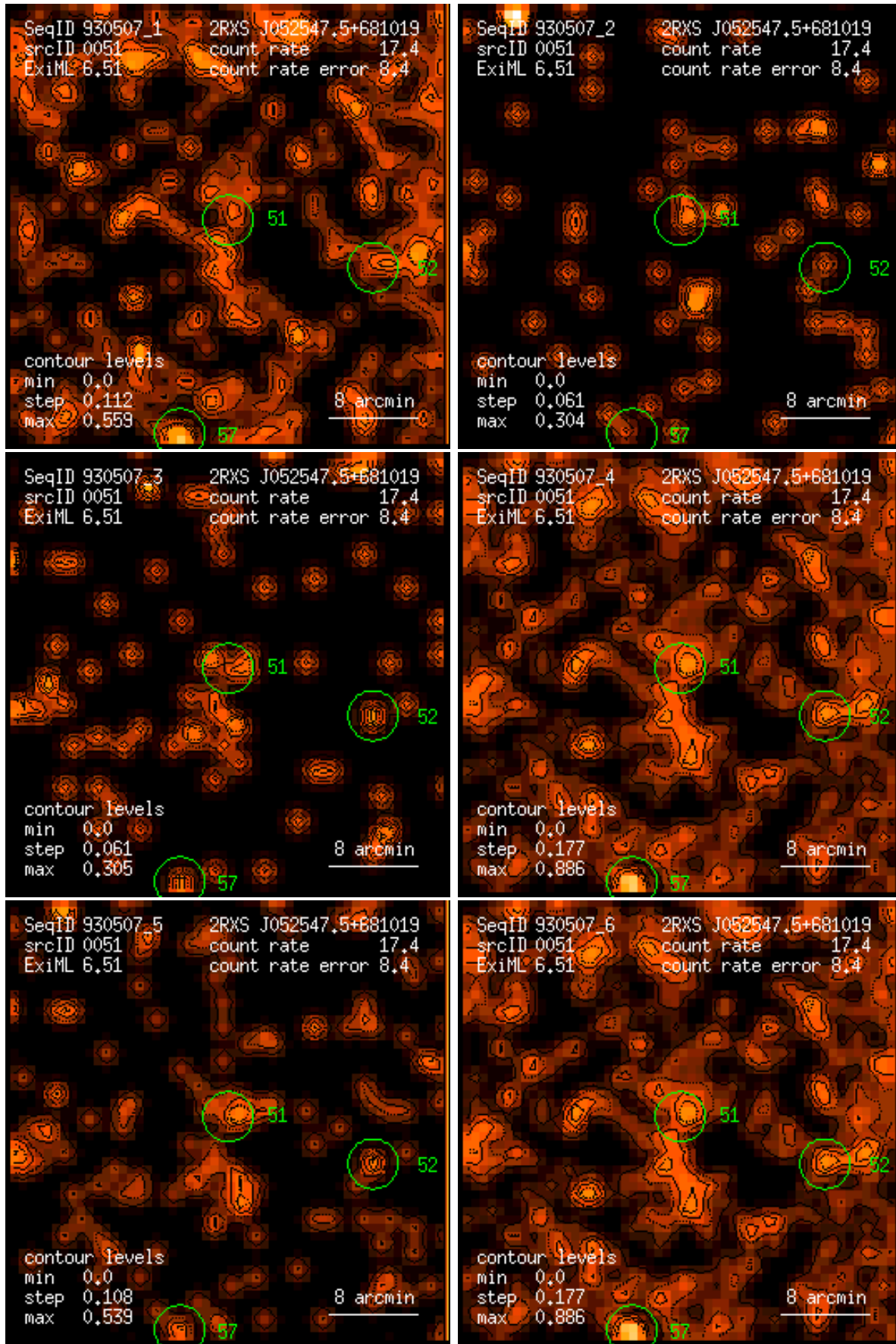
Figure 51: RASS 930507: detection 0051: band rate images, Gaussian filter: (1) PSPC channels 11 – 41, (2) 52 – 90, (3) 91 – 201, (4) 11 – 235, (5) 52 – 201, (6) 11 – 201. Broad band rates in counts/ks. Band rate contour levels in counts/ks/arcmin 2 .
