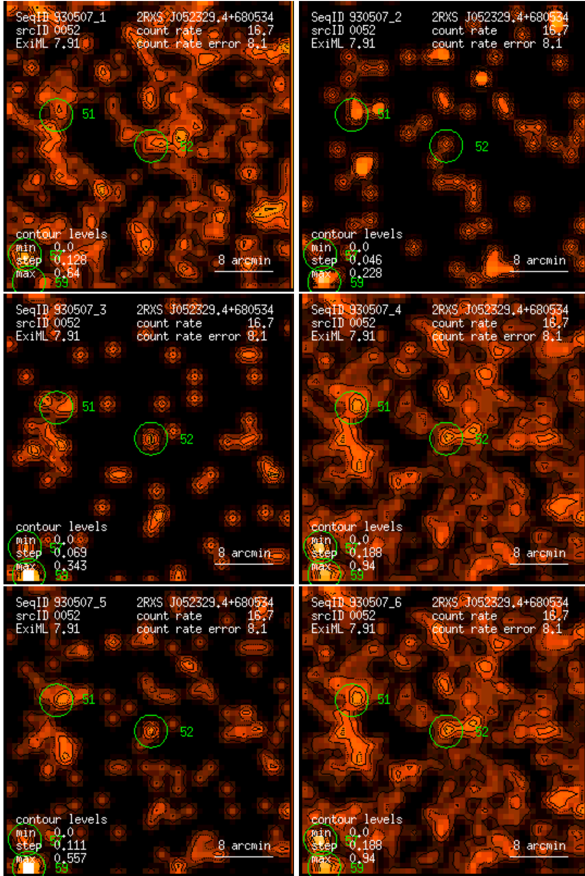
Figure 52: RASS 930507: detection 0052: band rate images, Gaussian filter: (1) PSPC channels 11 – 41, (2) 52 – 90, (3) 91 – 201, (4) 11 – 235, (5) 52 – 201, (6) 11 – 201. Broad band rates in counts/ks. Band rate contour levels in counts/ks/arcmin 2 .
