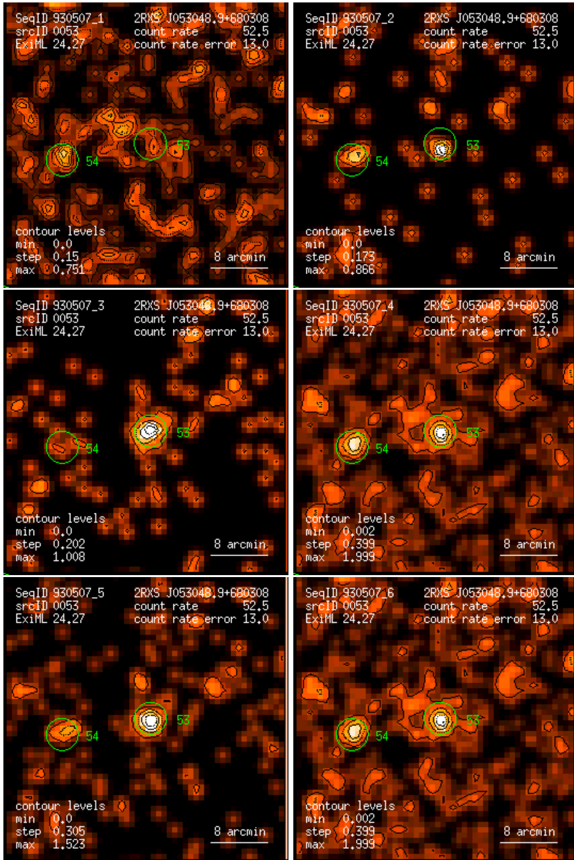
Figure 53: RASS 930507: detection 0053: band rate images, Gaussian filter: (1) PSPC channels 11 – 41, (2) 52 – 90, (3) 91 – 201, (4) 11 – 235, (5) 52 – 201, (6) 11 – 201. Broad band rates in counts/ks. Band rate contour levels in counts/ks/arcmin 2 .
