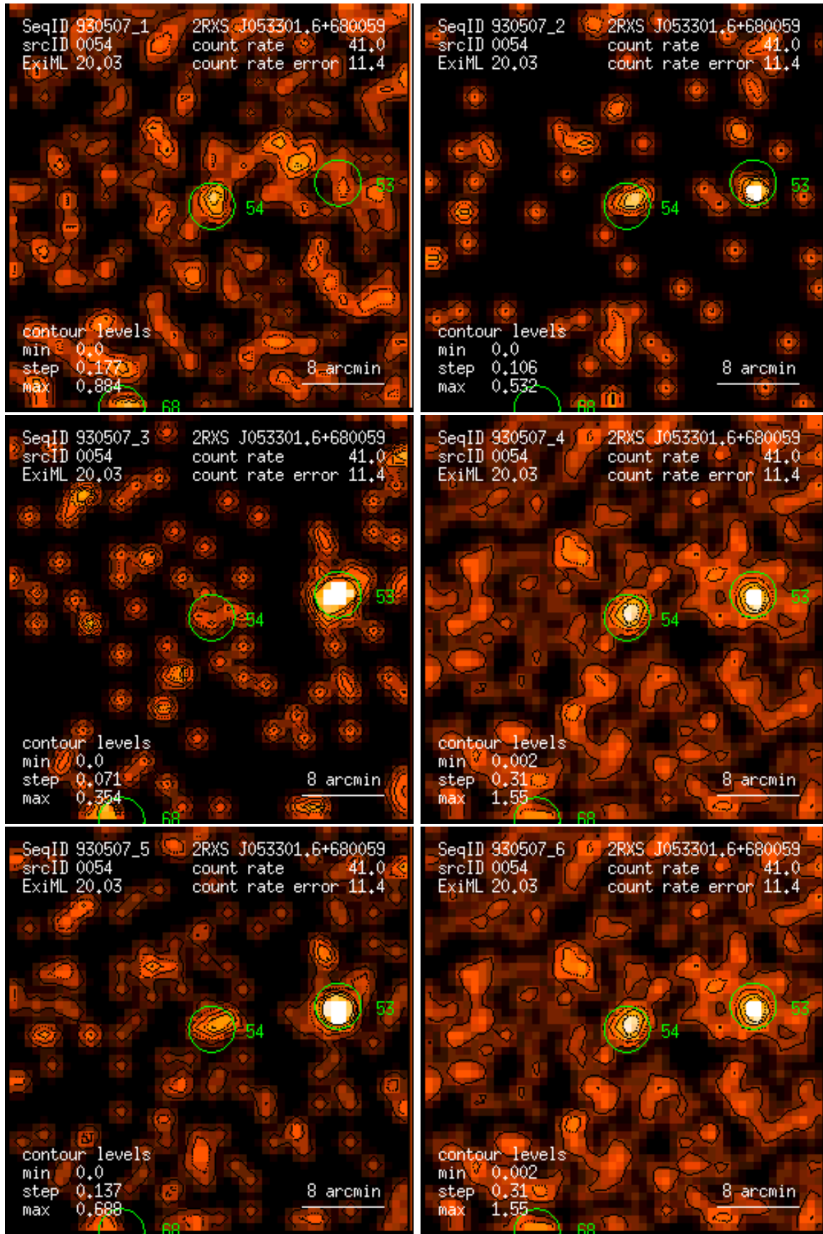
Figure 54: RASS 930507: detection 0054: band rate images, Gaussian filter: (1) PSPC channels 11 – 41, (2) 52 – 90, (3) 91 – 201, (4) 11 – 235, (5) 52 – 201, (6) 11 – 201. Broad band rates in counts/ks. Band rate contour levels in counts/ks/arcmin 2 .
