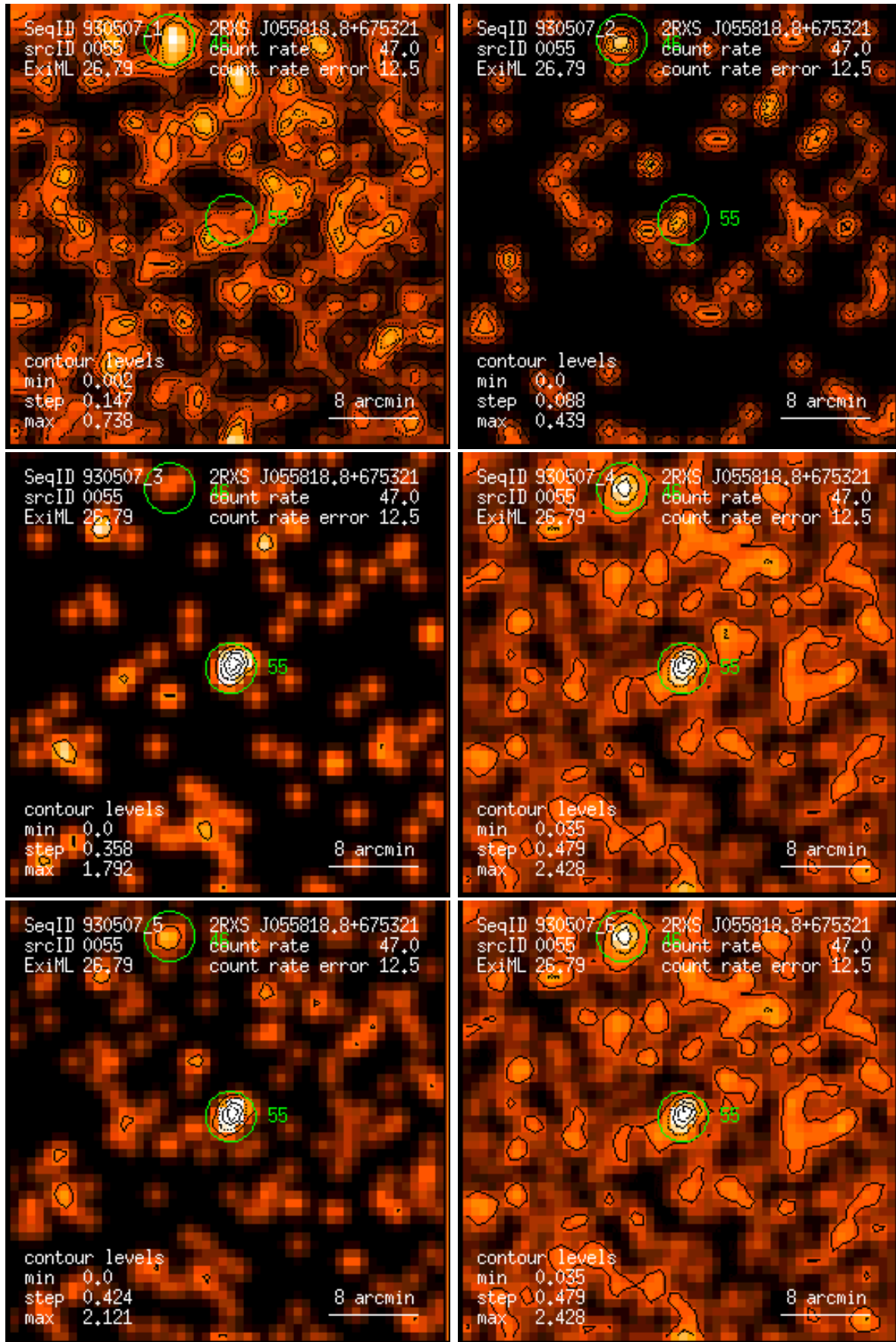
Figure 55: RASS 930507: detection 0055: band rate images, Gaussian filter: (1) PSPC channels 11 – 41, (2) 52 – 90, (3) 91 – 201, (4) 11 – 235, (5) 52 – 201, (6) 11 – 201. Broad band rates in counts/ks. Band rate contour levels in counts/ks/arcmin 2 .
