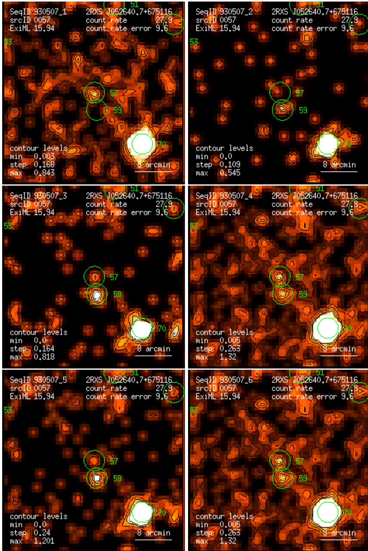
Figure 57: RASS 930507: detection 0057: band rate images, Gaussian filter: (1) PSPC channels 11 – 41, (2) 52 – 90, (3) 91 – 201, (4) 11 – 235, (5) 52 – 201, (6) 11 – 201. Broad band rates in counts/ks. Band rate contour levels in counts/ks/arcmin 2 .
