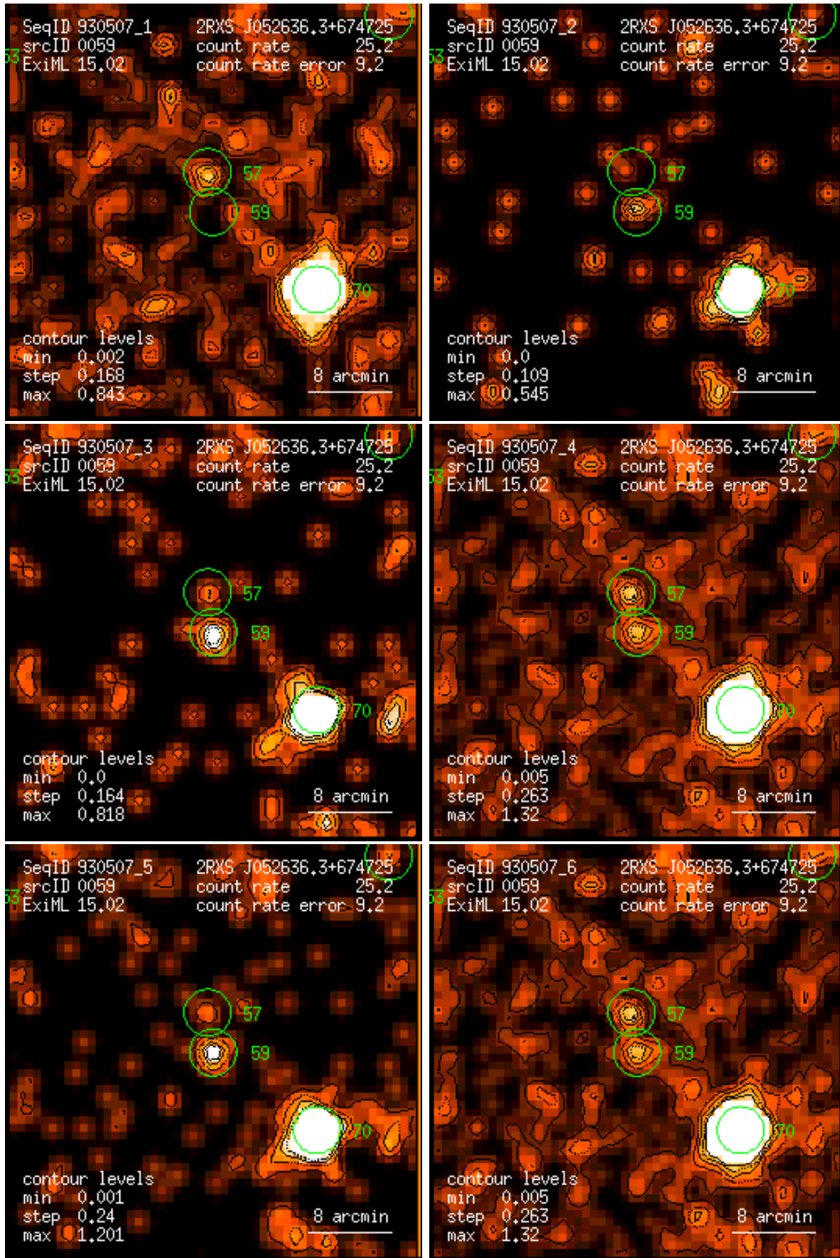
Figure 59: RASS 930507: detection 0059: band rate images, Gaussian filter: (1) PSPC channels 11 – 41, (2) 52 – 90, (3) 91 – 201, (4) 11 – 235, (5) 52 – 201, (6) 11 – 201. Broad band rates in counts/ks. Band rate contour levels in counts/ks/arcmin 2 .
