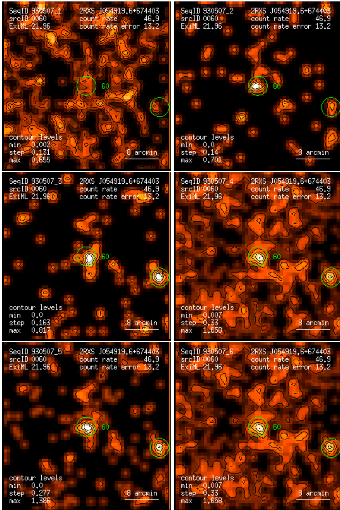
Figure 60: RASS 930507: detection 0060: band rate images, Gaussian filter: (1) PSPC channels 11 – 41, (2) 52 – 90, (3) 91 – 201, (4) 11 – 235, (5) 52 – 201, (6) 11 – 201. Broad band rates in counts/ks. Band rate contour levels in counts/ks/arcmin 2 .
