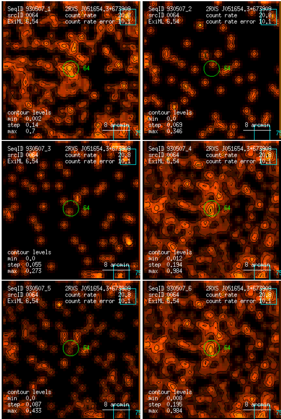
Figure 64: RASS 930507: detection 0064: band rate images, Gaussian filter: (1) PSPC channels 11 – 41, (2) 52 – 90, (3) 91 – 201, (4) 11 – 235, (5) 52 – 201, (6) 11 – 201. Broad band rates in counts/ks. Band rate contour levels in counts/ks/arcmin 2 .
