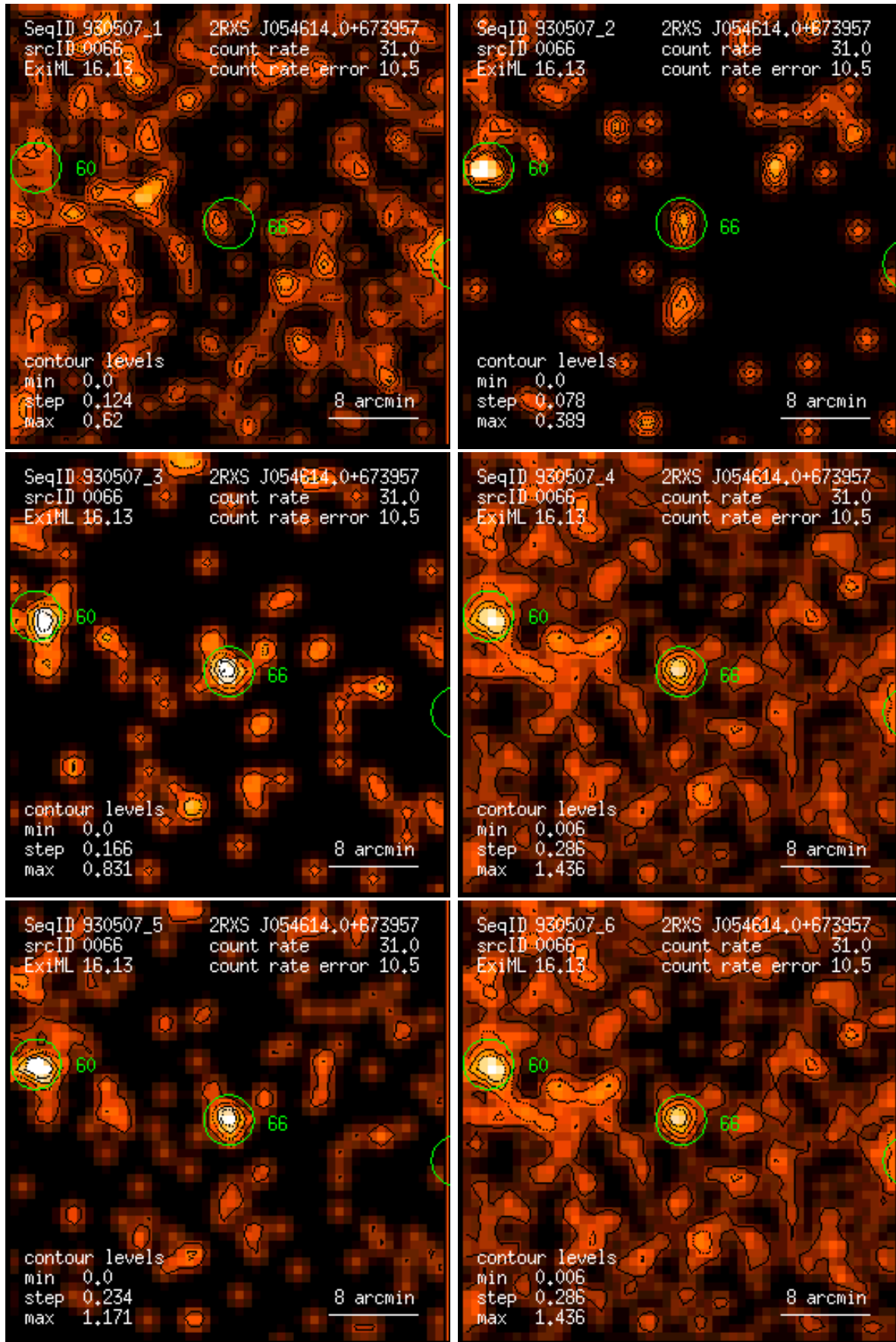
Figure 66: RASS 930507: detection 0066: band rate images, Gaussian filter: (1) PSPC channels 11 – 41, (2) 52 – 90, (3) 91 – 201, (4) 11 – 235, (5) 52 – 201, (6) 11 – 201. Broad band rates in counts/ks. Band rate contour levels in counts/ks/arcmin 2 .
