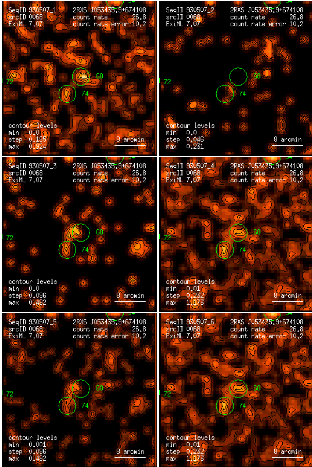
Figure 68: RASS 930507: detection 0068: band rate images, Gaussian filter: (1) PSPC channels 11 – 41, (2) 52 – 90, (3) 91 – 201, (4) 11 – 235, (5) 52 – 201, (6) 11 – 201. Broad band rates in counts/ks. Band rate contour levels in counts/ks/arcmin 2 .
