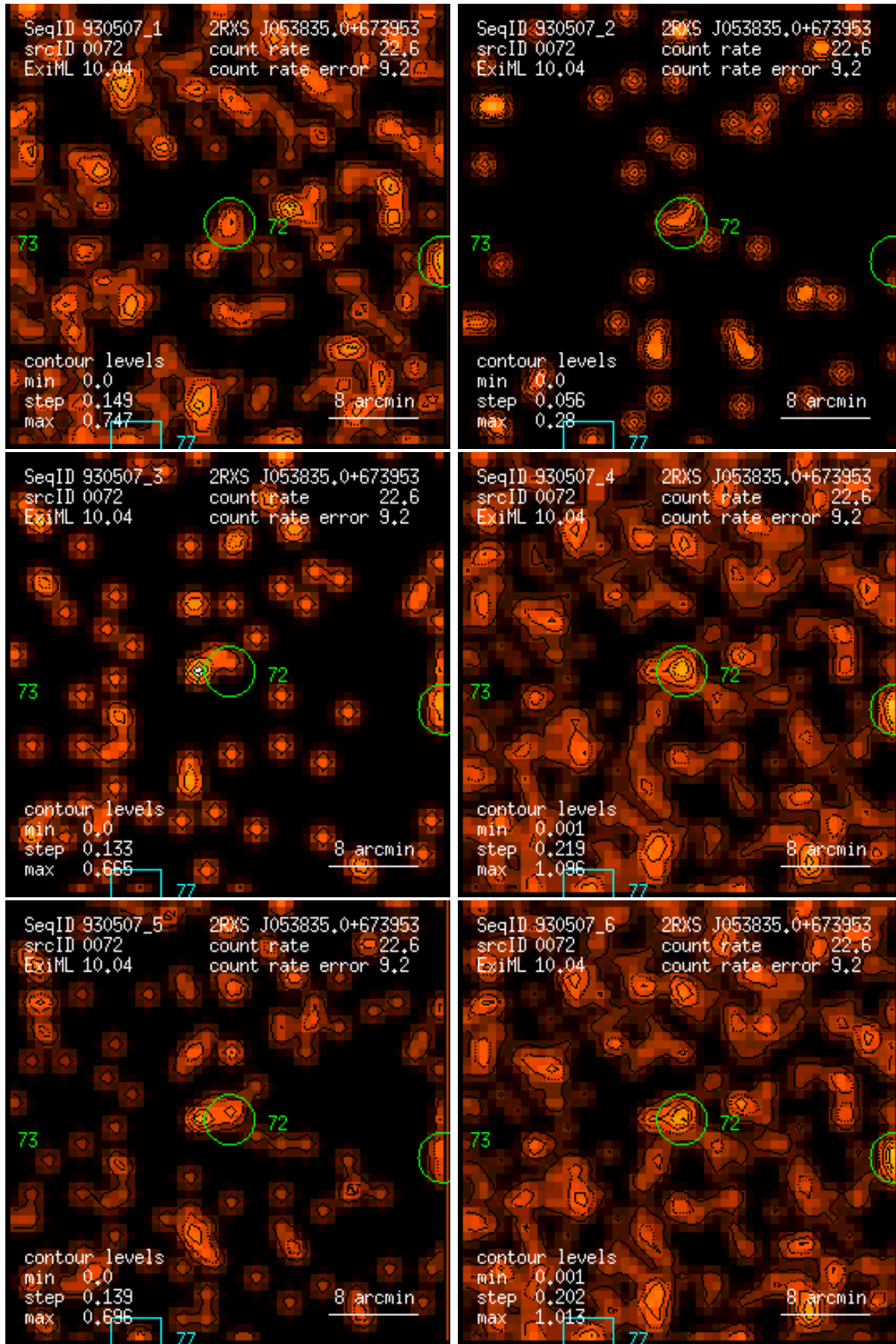
Figure 72: RASS 930507: detection 0072: band rate images, Gaussian filter: (1) PSPC channels 11 – 41, (2) 52 – 90, (3) 91 – 201, (4) 11 – 235, (5) 52 – 201, (6) 11 – 201. Broad band rates in counts/ks. Band rate contour levels in counts/ks/arcmin 2 .
