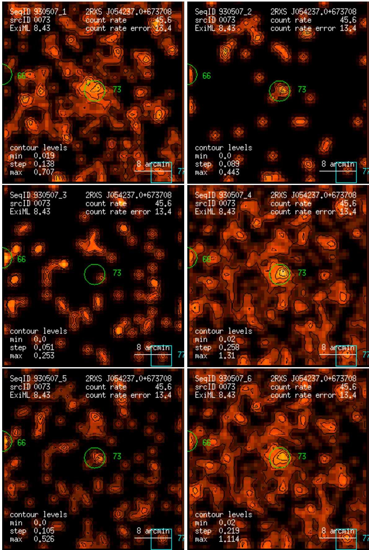
Figure 73: RASS 930507: detection 0073: band rate images, Gaussian filter: (1) PSPC channels 11 – 41, (2) 52 – 90, (3) 91 – 201, (4) 11 – 235, (5) 52 – 201, (6) 11 – 201. Broad band rates in counts/ks. Band rate contour levels in counts/ks/arcmin 2 .
