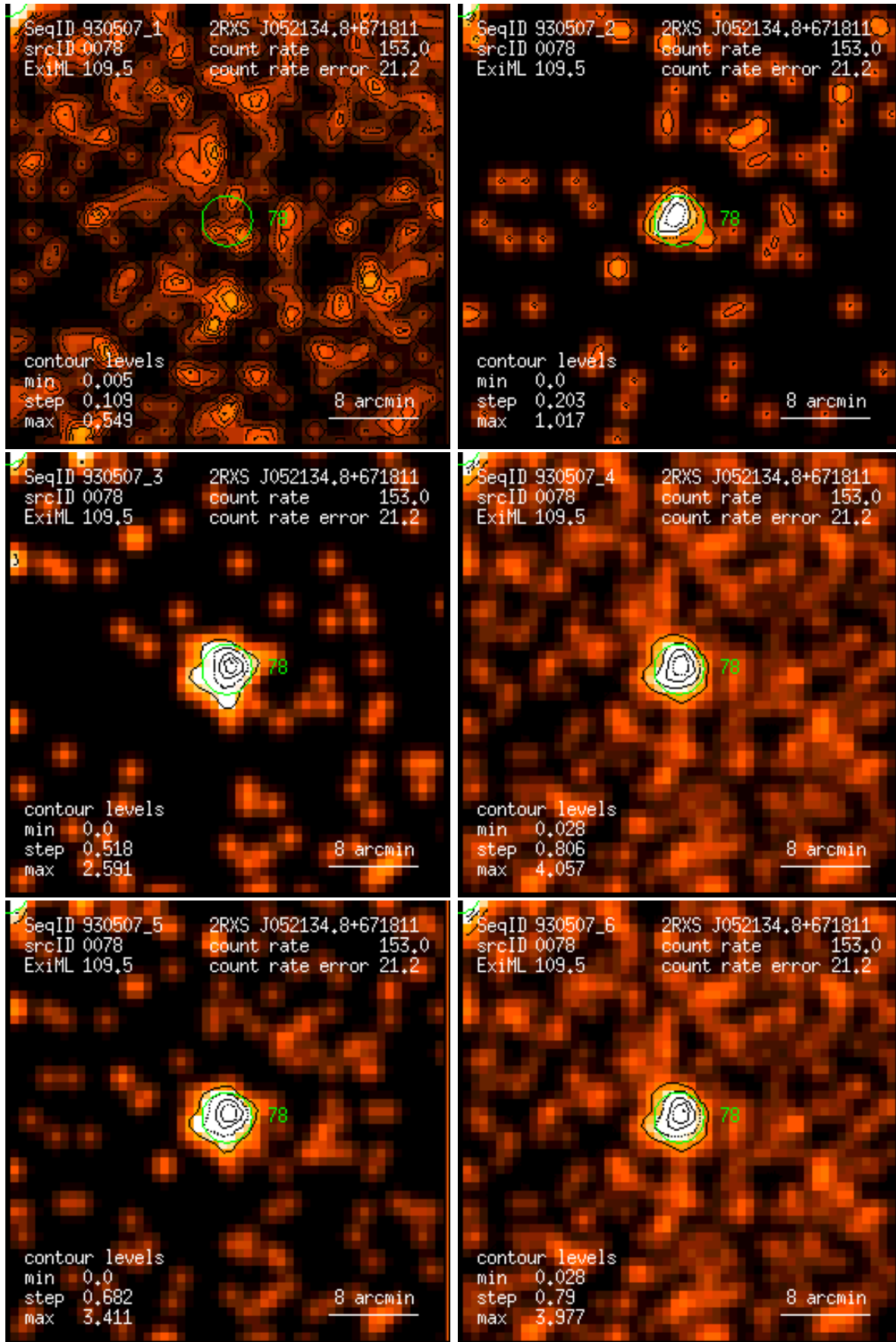
Figure 78: RASS 930507: detection 0078: band rate images, Gaussian filter: (1) PSPC channels 11 – 41, (2) 52 – 90, (3) 91 – 201, (4) 11 – 235, (5) 52 – 201, (6) 11 – 201. Broad band rates in counts/ks. Band rate contour levels in counts/ks/arcmin 2 .
