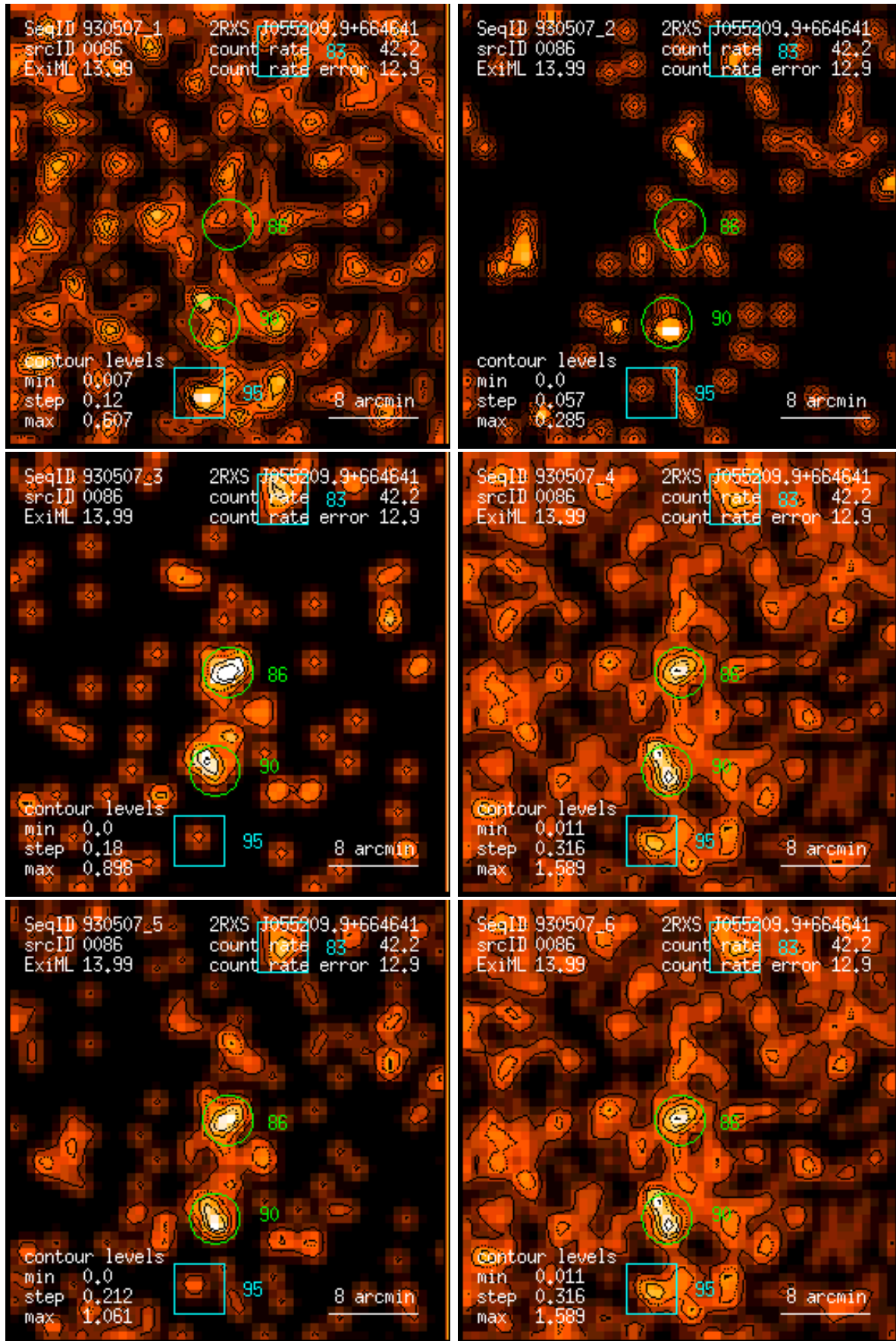
Figure 86: RASS 930507: detection 0086: band rate images, Gaussian filter: (1) PSPC channels 11 – 41, (2) 52 – 90, (3) 91 – 201, (4) 11 – 235, (5) 52 – 201, (6) 11 – 201. Broad band rates in counts/ks. Band rate contour levels in counts/ks/arcmin 2 .
