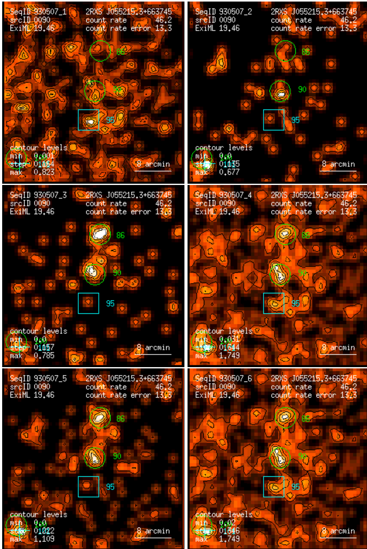
Figure 90: RASS 930507: detection 0090: band rate images, Gaussian filter: (1) PSPC channels 11 – 41, (2) 52 – 90, (3) 91 – 201, (4) 11 – 235, (5) 52 – 201, (6) 11 – 201. Broad band rates in counts/ks. Band rate contour levels in counts/ks/arcmin 2 .
