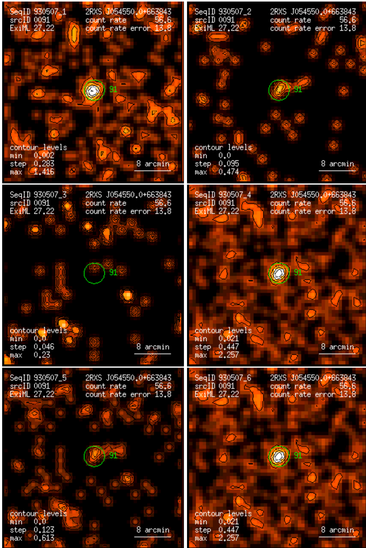
Figure 91: RASS 930507: detection 0091: band rate images, Gaussian filter: (1) PSPC channels 11 – 41, (2) 52 – 90, (3) 91 – 201, (4) 11 – 235, (5) 52 – 201, (6) 11 – 201. Broad band rates in counts/ks. Band rate contour levels in counts/ks/arcmin 2 .
