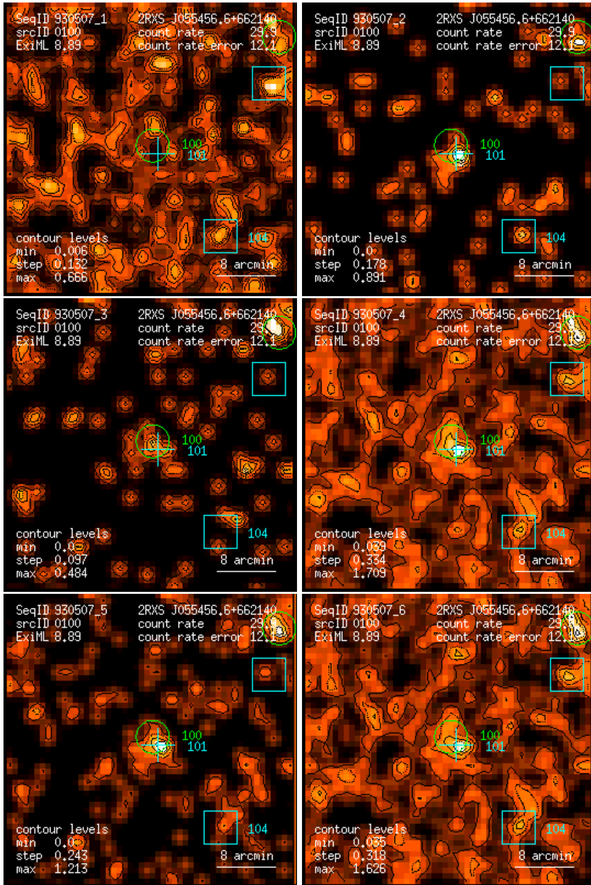
Figure 100: RASS 930507: detection 0100: band rate images, Gaussian filter: (1) PSPC channels 11 – 41, (2) 52 – 90, (3) 91 – 201, (4) 11 – 235, (5) 52 – 201, (6) 11 – 201. Broad band rates in counts/ks. Band rate contour levels in counts/ks/arcmin 2 .
