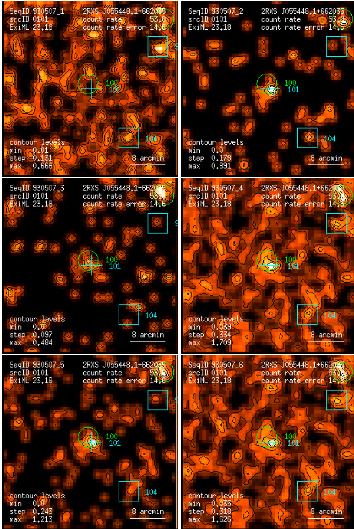
Figure 101: RASS 930507: detection 0101: band rate images, Gaussian filter: (1) PSPC channels 11 – 41, (2) 52 – 90, (3) 91 – 201, (4) 11 – 235, (5) 52 – 201, (6) 11 – 201. Broad band rates in counts/ks. Band rate contour levels in counts/ks/arcmin 2 .
