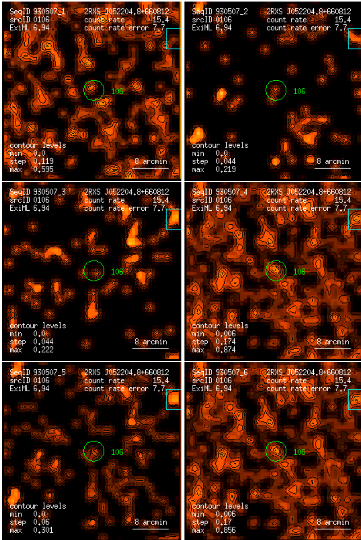
Figure 106: RASS 930507: detection 0106: band rate images, Gaussian filter: (1) PSPC channels 11 – 41, (2) 52 – 90, (3) 91 – 201, (4) 11 – 235, (5) 52 – 201, (6) 11 – 201. Broad band rates in counts/ks. Band rate contour levels in counts/ks/arcmin 2 .
