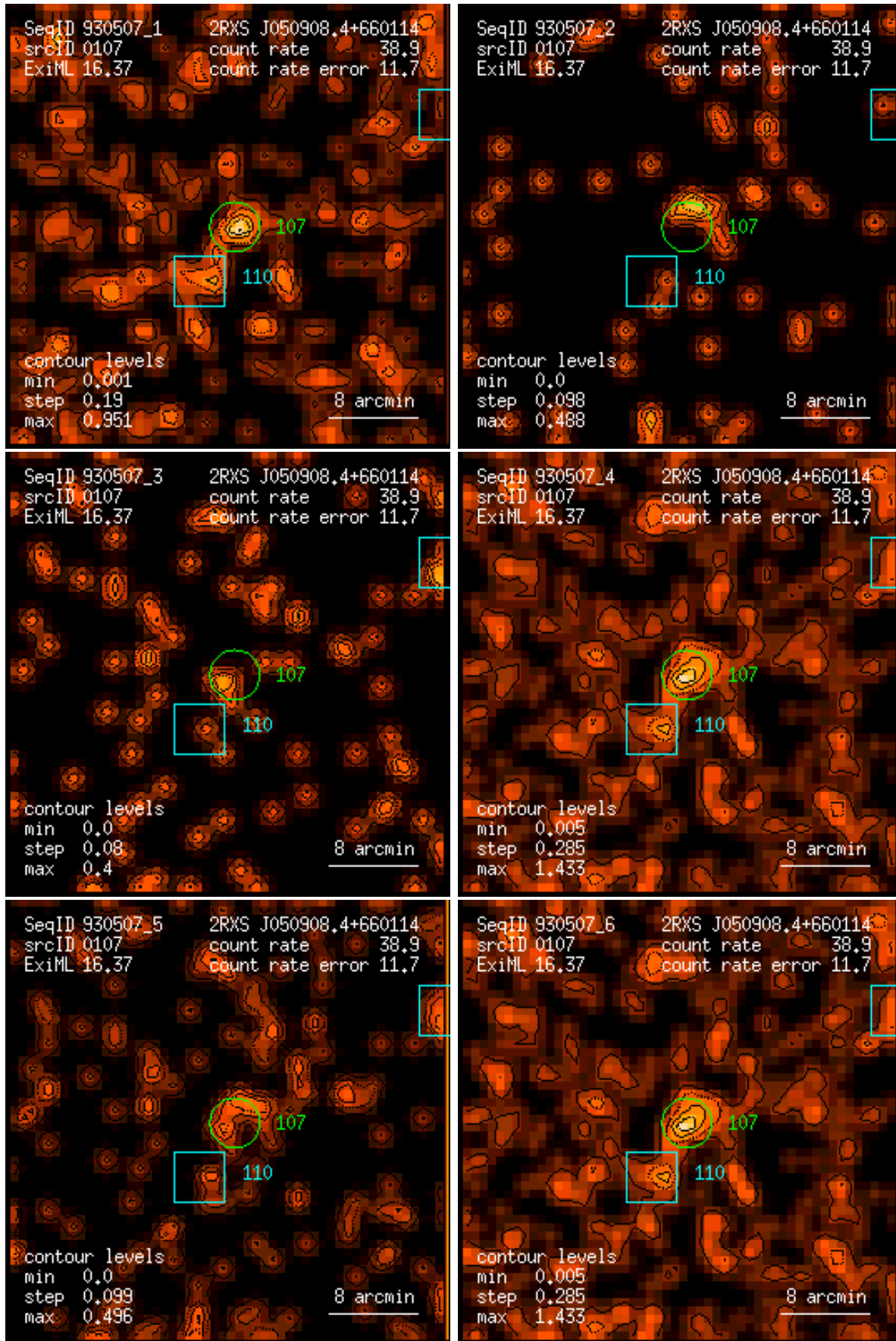
Figure 107: RASS 930507: detection 0107: band rate images, Gaussian filter: (1) PSPC channels 11 – 41, (2) 52 – 90, (3) 91 – 201, (4) 11 – 235, (5) 52 – 201, (6) 11 – 201. Broad band rates in counts/ks. Band rate contour levels in counts/ks/arcmin 2 .
