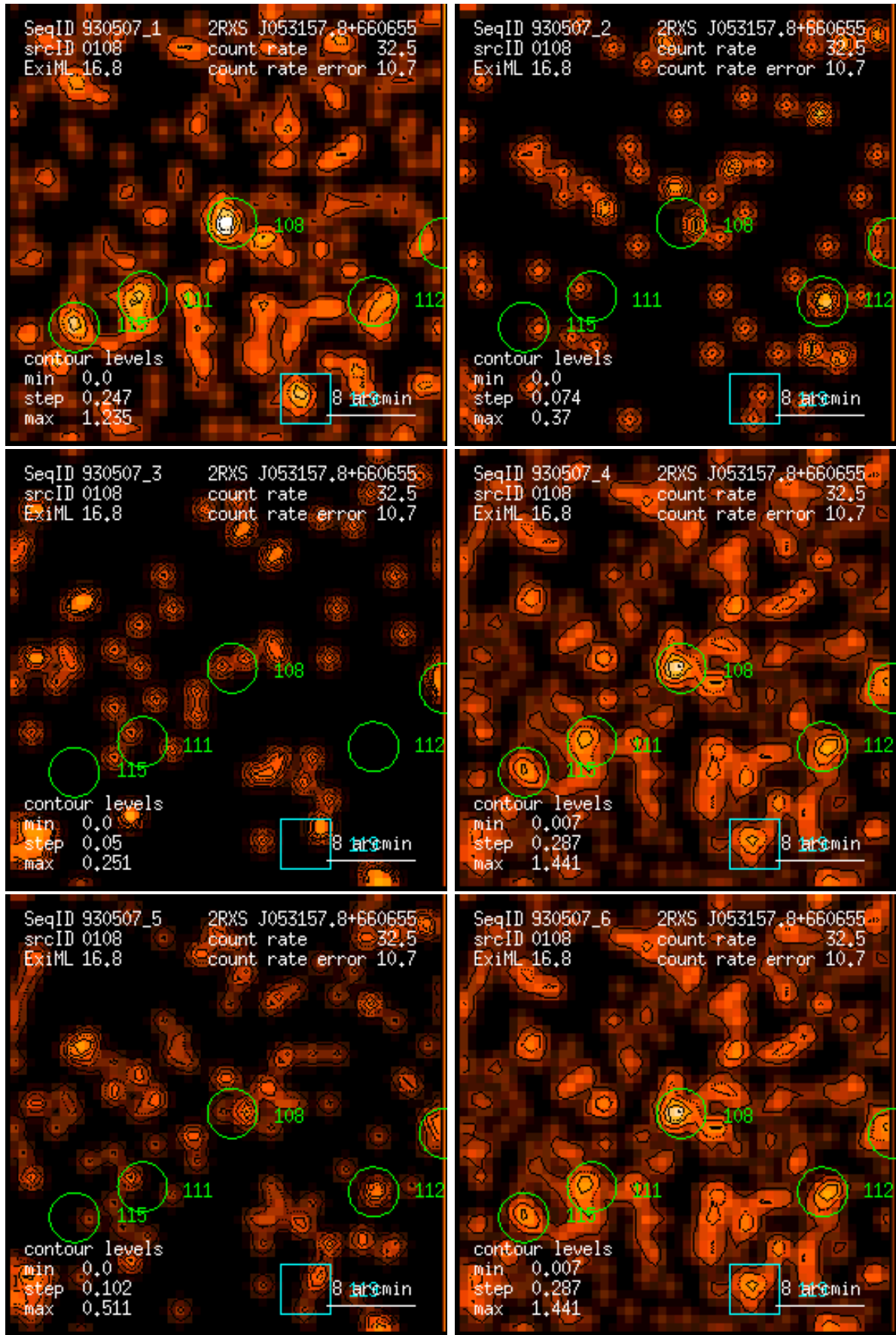
Figure 108: RASS 930507: detection 0108: band rate images, Gaussian filter: (1) PSPC channels 11 – 41, (2) 52 – 90, (3) 91 – 201, (4) 11 – 235, (5) 52 – 201, (6) 11 – 201. Broad band rates in counts/ks. Band rate contour levels in counts/ks/arcmin 2 .
