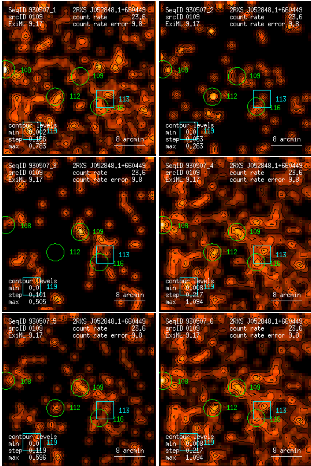
Figure 109: RASS 930507: detection 0109: band rate images, Gaussian filter: (1) PSPC channels 11 – 41, (2) 52 – 90, (3) 91 – 201, (4) 11 – 235, (5) 52 – 201, (6) 11 – 201. Broad band rates in counts/ks. Band rate contour levels in counts/ks/arcmin 2 .
