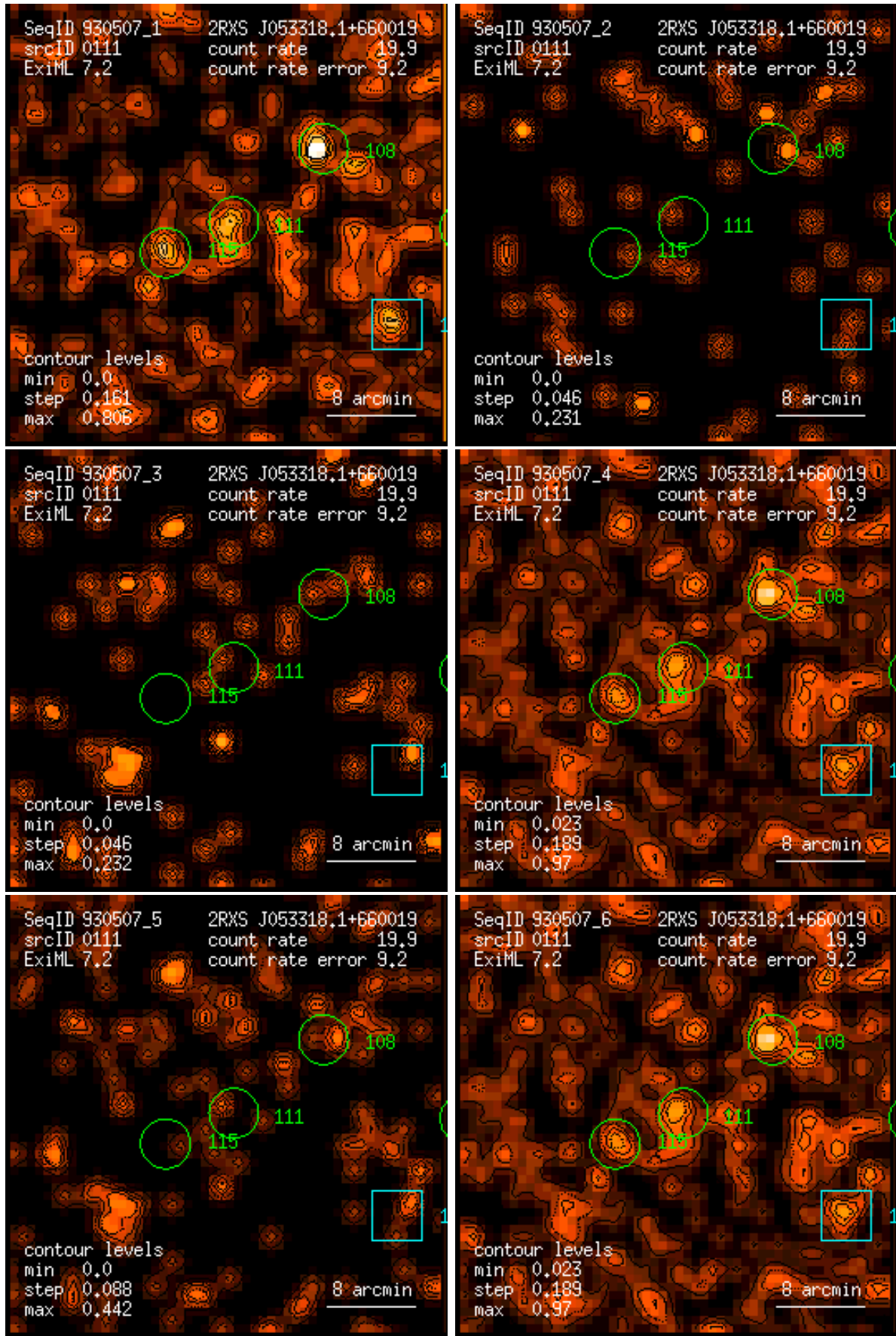
Figure 111: RASS 930507: detection 0111: band rate images, Gaussian filter: (1) PSPC channels 11 – 41, (2) 52 – 90, (3) 91 – 201, (4) 11 – 235, (5) 52 – 201, (6) 11 – 201. Broad band rates in counts/ks. Band rate contour levels in counts/ks/arcmin 2 .
