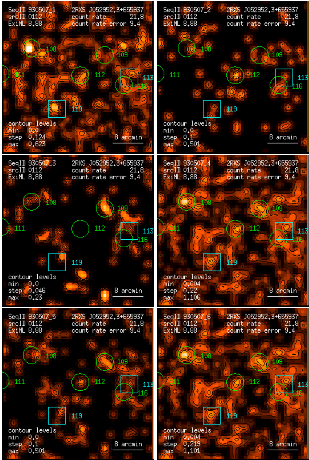
Figure 112: RASS 930507: detection 0112: band rate images, Gaussian filter: (1) PSPC channels 11 – 41, (2) 52 – 90, (3) 91 – 201, (4) 11 – 235, (5) 52 – 201, (6) 11 – 201. Broad band rates in counts/ks. Band rate contour levels in counts/ks/arcmin 2 .
