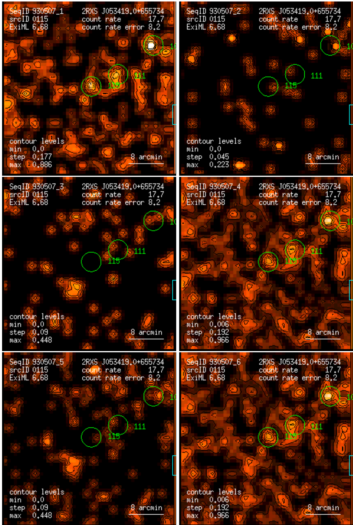
Figure 115: RASS 930507: detection 0115: band rate images, Gaussian filter: (1) PSPC channels 11 – 41, (2) 52 – 90, (3) 91 – 201, (4) 11 – 235, (5) 52 – 201, (6) 11 – 201. Broad band rates in counts/ks. Band rate contour levels in counts/ks/arcmin 2 .
