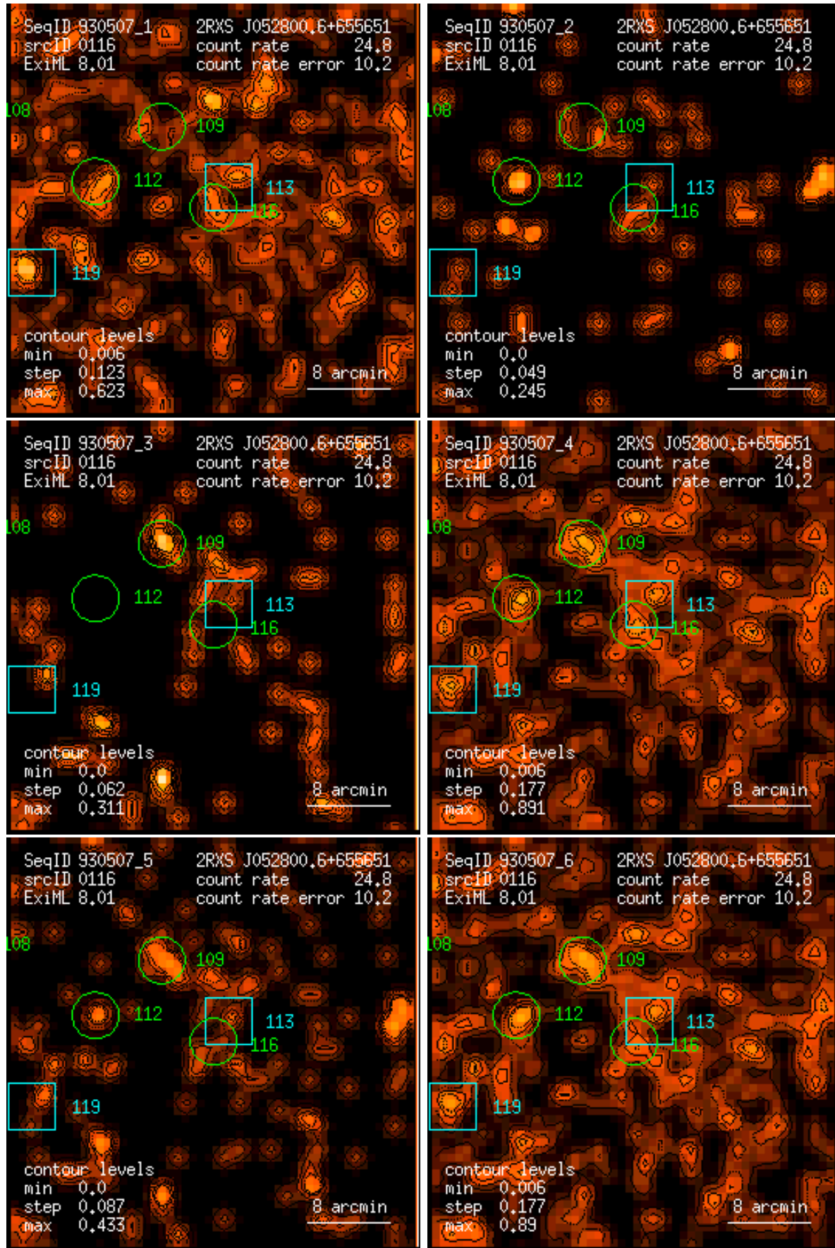
Figure 116: RASS 930507: detection 0116: band rate images, Gaussian filter: (1) PSPC channels 11 – 41, (2) 52 – 90, (3) 91 – 201, (4) 11 – 235, (5) 52 – 201, (6) 11 – 201. Broad band rates in counts/ks. Band rate contour levels in counts/ks/arcmin 2 .
