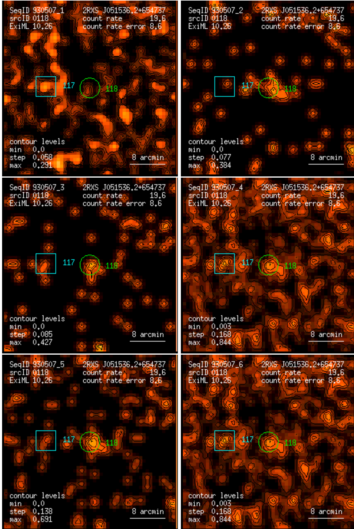
Figure 118: RASS 930507: detection 0118: band rate images, Gaussian filter: (1) PSPC channels 11 – 41, (2) 52 – 90, (3) 91 – 201, (4) 11 – 235, (5) 52 – 201, (6) 11 – 201. Broad band rates in counts/ks. Band rate contour levels in counts/ks/arcmin 2 .
