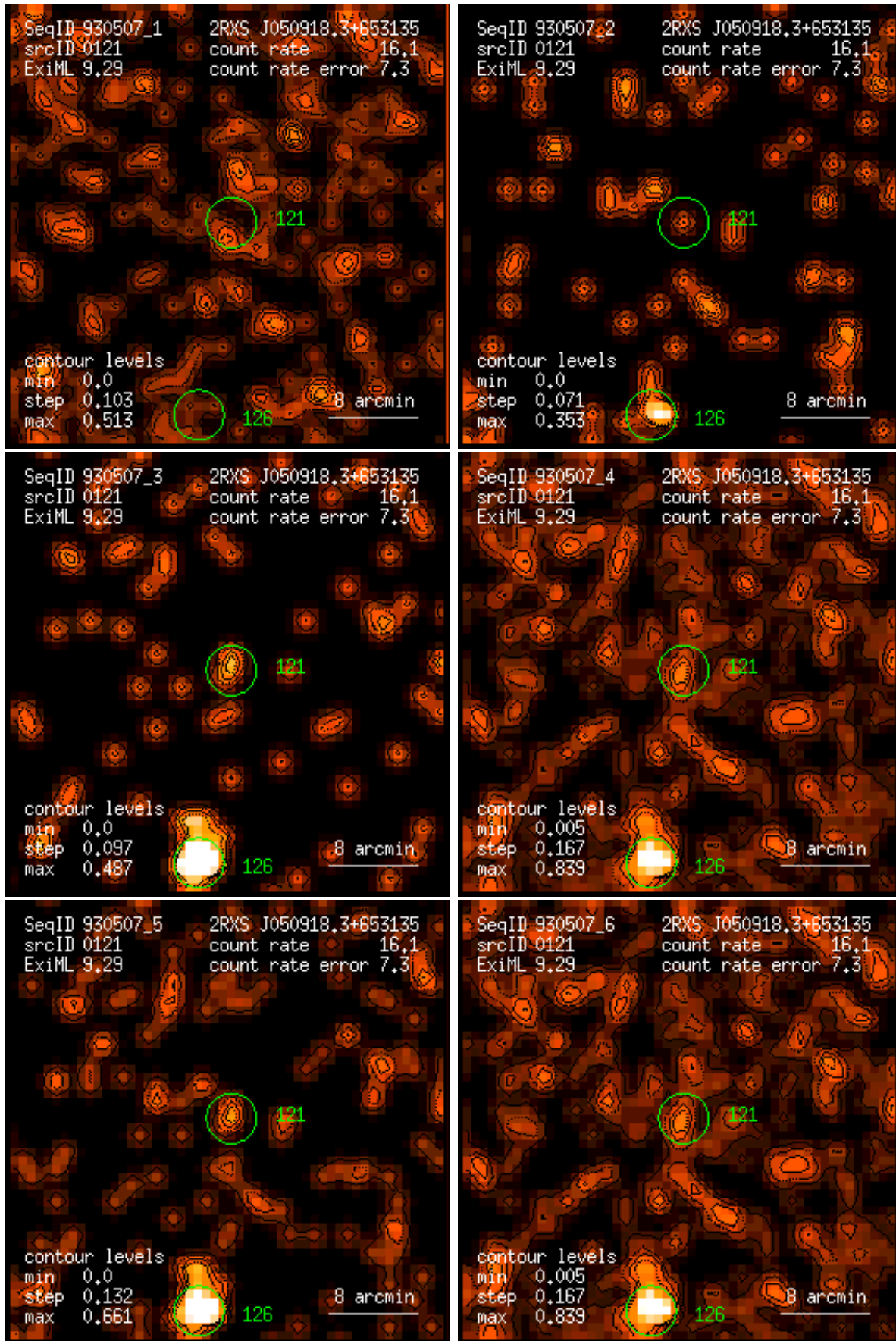
Figure 121: RASS 930507: detection 0121: band rate images, Gaussian filter: (1) PSPC channels 11 – 41, (2) 52 – 90, (3) 91 – 201, (4) 11 – 235, (5) 52 – 201, (6) 11 – 201. Broad band rates in counts/ks. Band rate contour levels in counts/ks/arcmin 2 .
