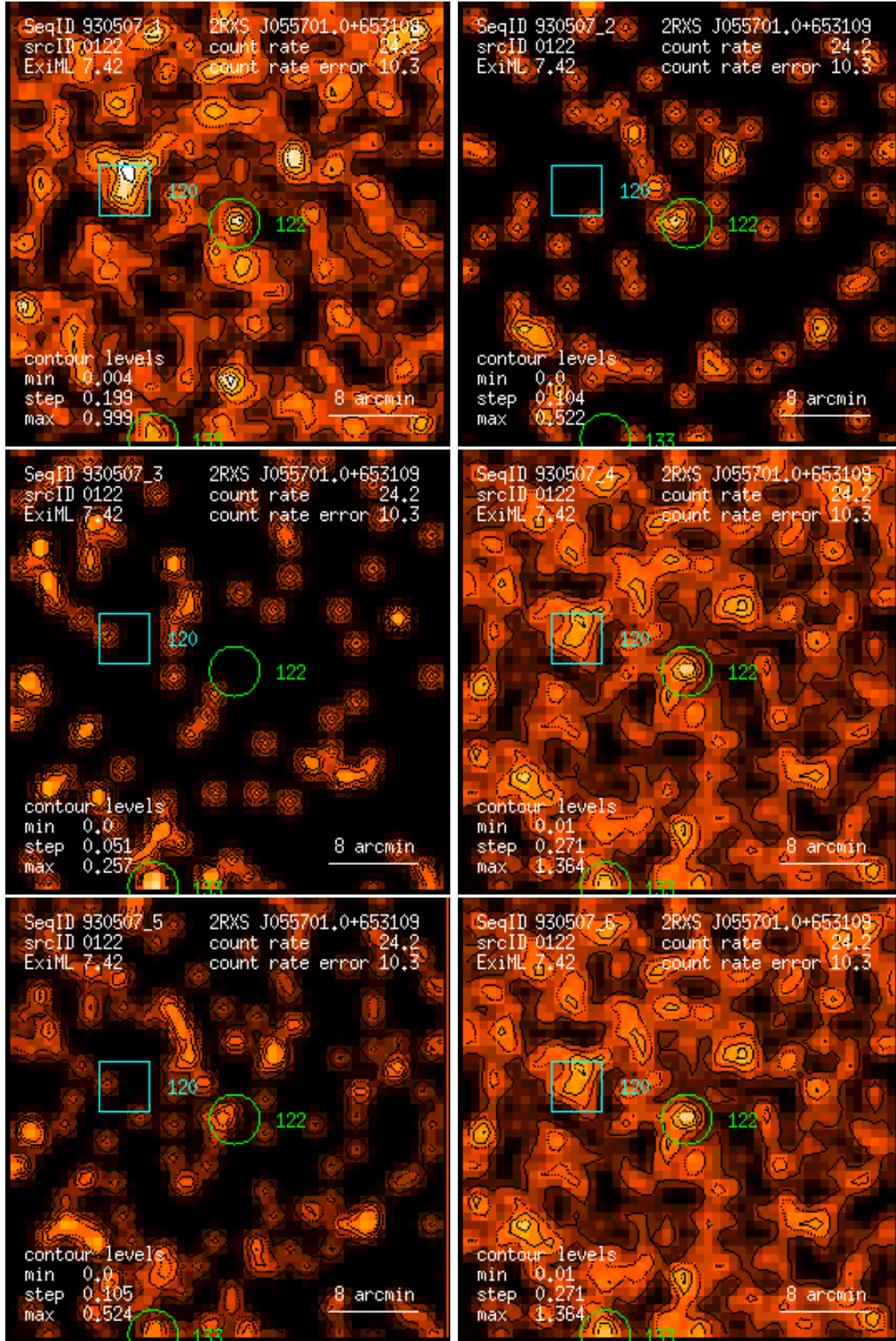
Figure 122: RASS 930507: detection 0122: band rate images, Gaussian filter: (1) PSPC channels 11 – 41, (2) 52 – 90, (3) 91 – 201, (4) 11 – 235, (5) 52 – 201, (6) 11 – 201. Broad band rates in counts/ks. Band rate contour levels in counts/ks/arcmin 2 .
