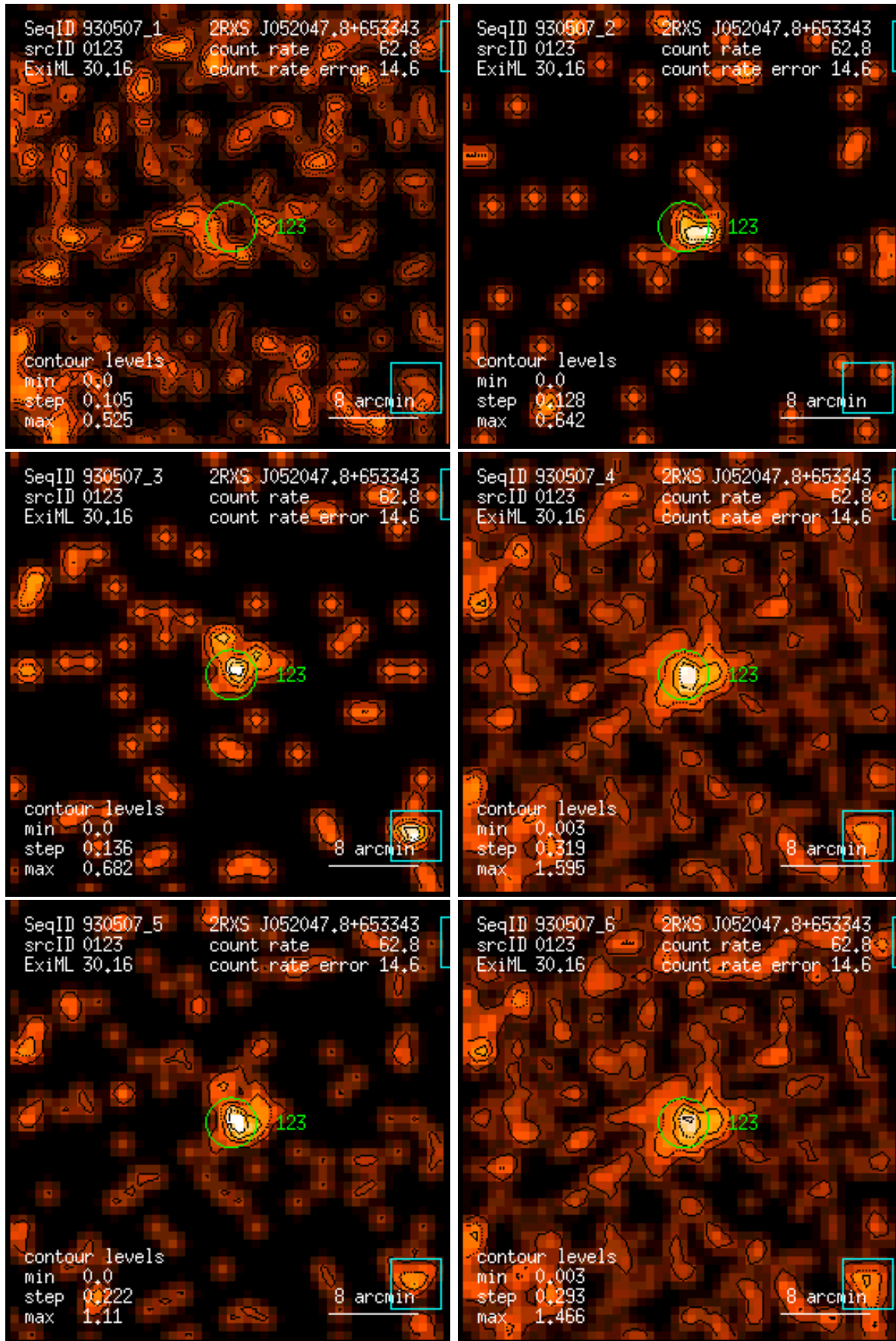
Figure 123: RASS 930507: detection 0123: band rate images, Gaussian filter: (1) PSPC channels 11 – 41, (2) 52 – 90, (3) 91 – 201, (4) 11 – 235, (5) 52 – 201, (6) 11 – 201. Broad band rates in counts/ks. Band rate contour levels in counts/ks/arcmin 2 .
