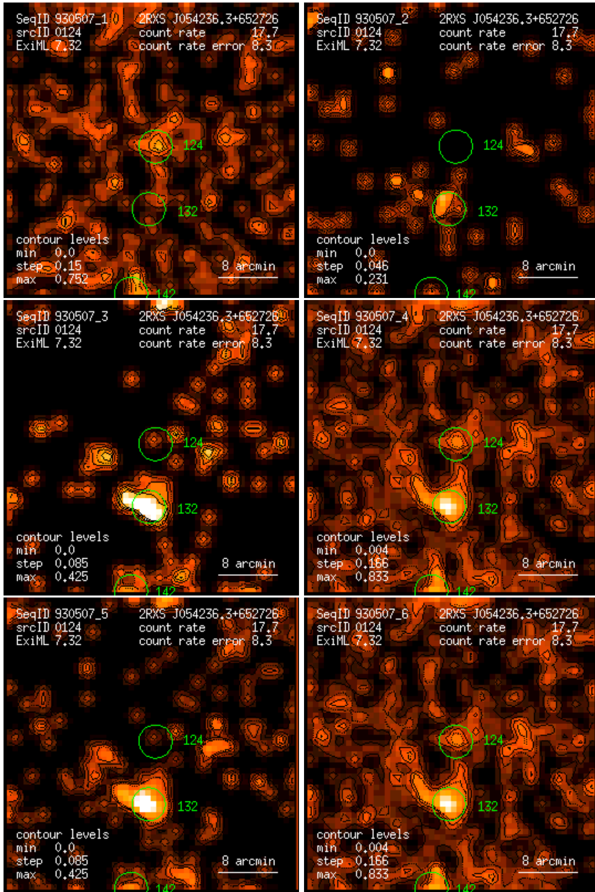
Figure 124: RASS 930507: detection 0124: band rate images, Gaussian filter: (1) PSPC channels 11 – 41, (2) 52 – 90, (3) 91 – 201, (4) 11 – 235, (5) 52 – 201, (6) 11 – 201. Broad band rates in counts/ks. Band rate contour levels in counts/ks/arcmin 2 .
