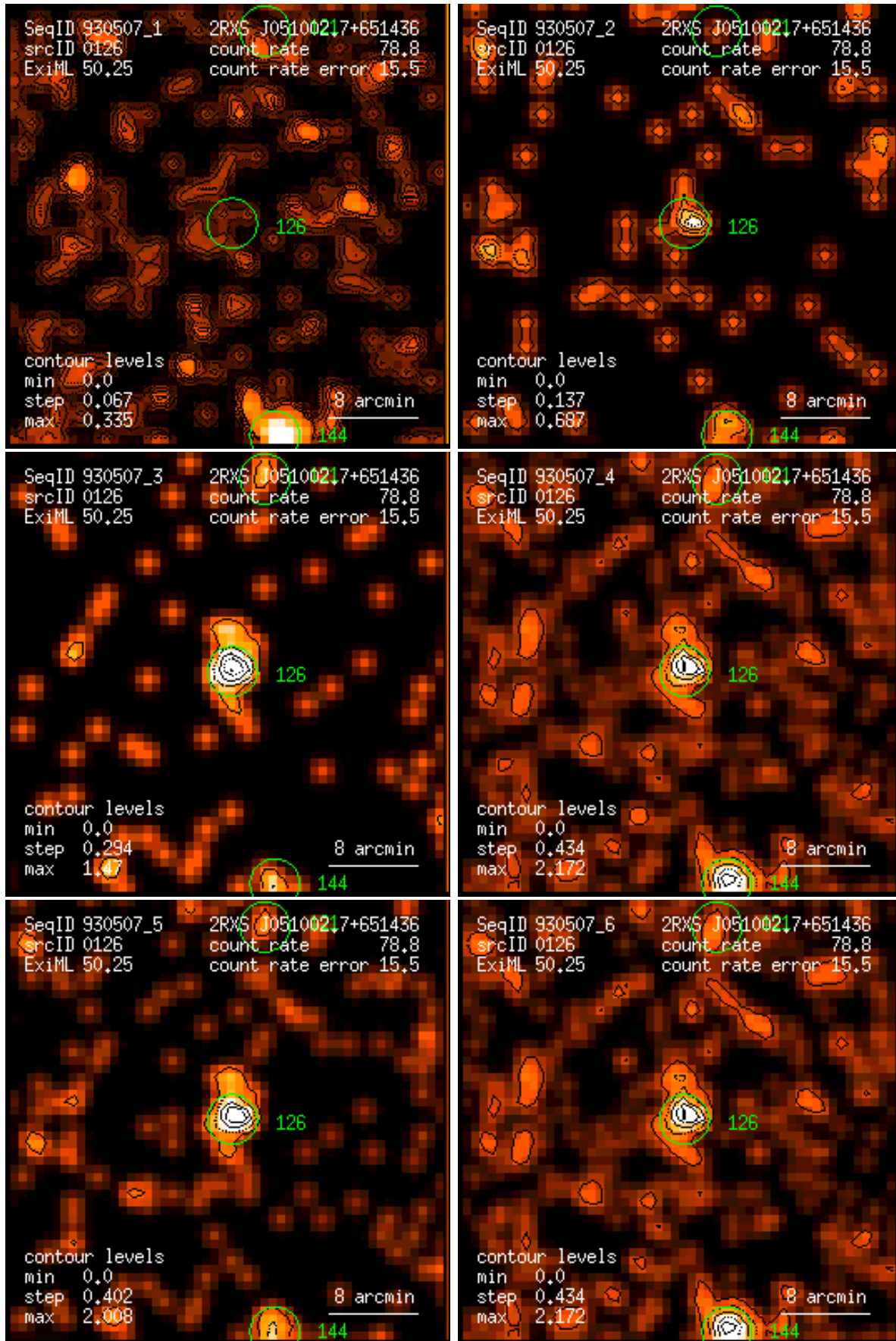
Figure 126: RASS 930507: detection 0126: band rate images, Gaussian filter: (1) PSPC channels 11 – 41, (2) 52 – 90, (3) 91 – 201, (4) 11 – 235, (5) 52 – 201, (6) 11 – 201. Broad band rates in counts/ks. Band rate contour levels in counts/ks/arcmin 2 .
