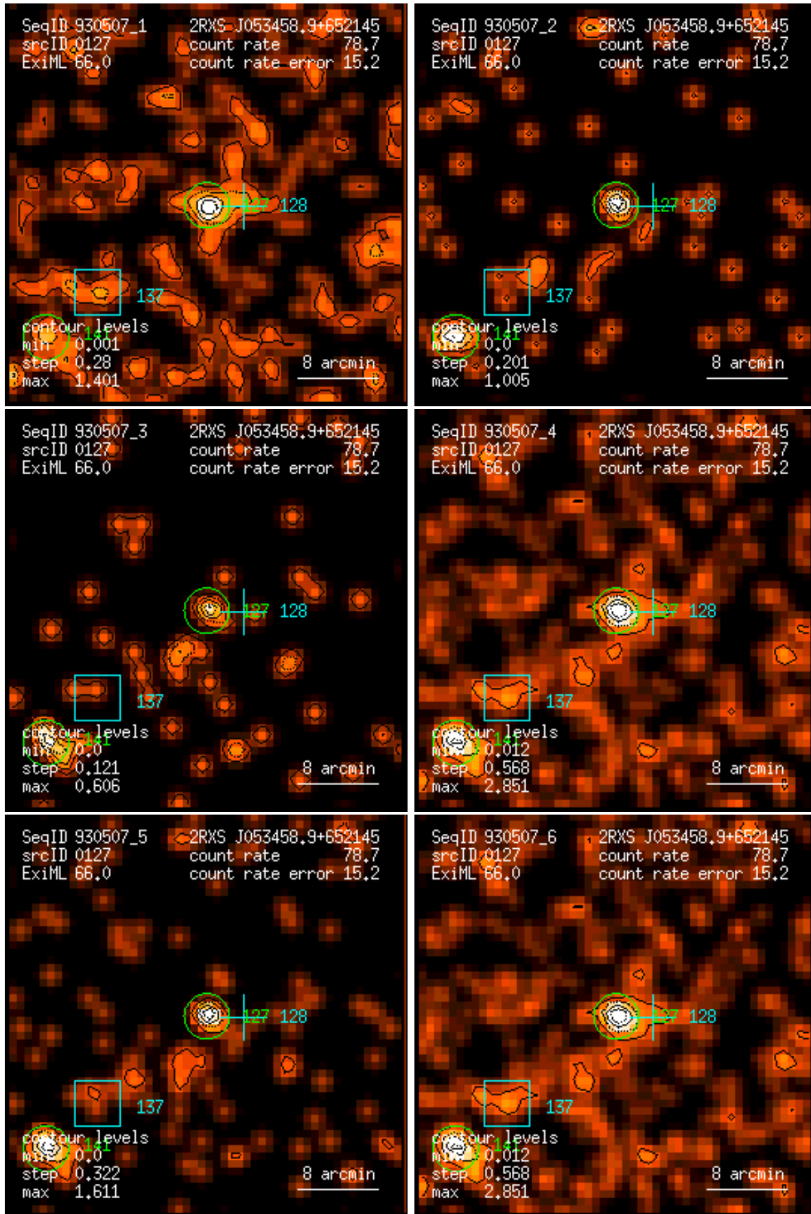
Figure 127: RASS 930507: detection 0127: band rate images, Gaussian filter: (1) PSPC channels 11 – 41, (2) 52 – 90, (3) 91 – 201, (4) 11 – 235, (5) 52 – 201, (6) 11 – 201. Broad band rates in counts/ks. Band rate contour levels in counts/ks/arcmin 2 .
