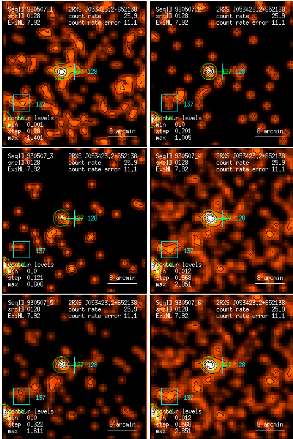
Figure 128: RASS 930507: detection 0128: band rate images, Gaussian filter: (1) PSPC channels 11 – 41, (2) 52 – 90, (3) 91 – 201, (4) 11 – 235, (5) 52 – 201, (6) 11 – 201. Broad band rates in counts/ks. Band rate contour levels in counts/ks/arcmin 2 .
