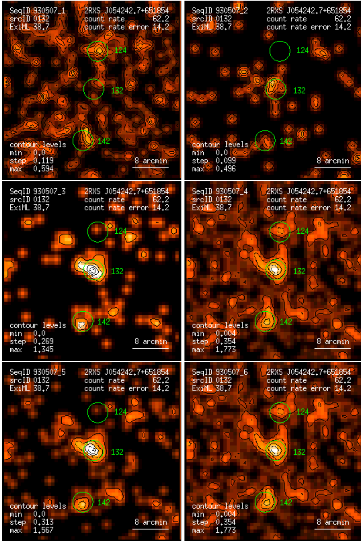
Figure 132: RASS 930507: detection 0132: band rate images, Gaussian filter: (1) PSPC channels 11 – 41, (2) 52 – 90, (3) 91 – 201, (4) 11 – 235, (5) 52 – 201, (6) 11 – 201. Broad band rates in counts/ks. Band rate contour levels in counts/ks/arcmin 2 .
