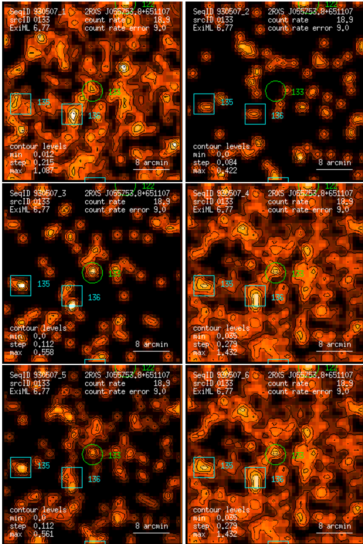
Figure 133: RASS 930507: detection 0133: band rate images, Gaussian filter: (1) PSPC channels 11 – 41, (2) 52 – 90, (3) 91 – 201, (4) 11 – 235, (5) 52 – 201, (6) 11 – 201. Broad band rates in counts/ks. Band rate contour levels in counts/ks/arcmin 2 .
