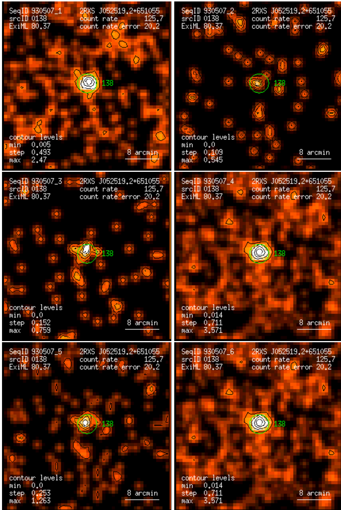
Figure 138: RASS 930507: detection 0138: band rate images, Gaussian filter: (1) PSPC channels 11 – 41, (2) 52 – 90, (3) 91 – 201, (4) 11 – 235, (5) 52 – 201, (6) 11 – 201. Broad band rates in counts/ks. Band rate contour levels in counts/ks/arcmin 2 .
