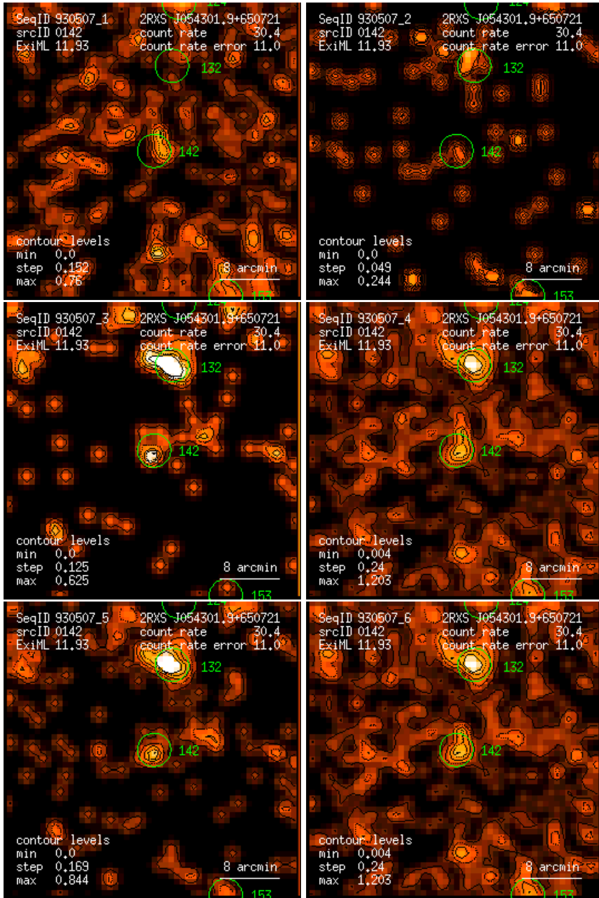
Figure 142: RASS 930507: detection 0142: band rate images, Gaussian filter: (1) PSPC channels 11 – 41, (2) 52 – 90, (3) 91 – 201, (4) 11 – 235, (5) 52 – 201, (6) 11 – 201. Broad band rates in counts/ks. Band rate contour levels in counts/ks/arcmin 2 .
