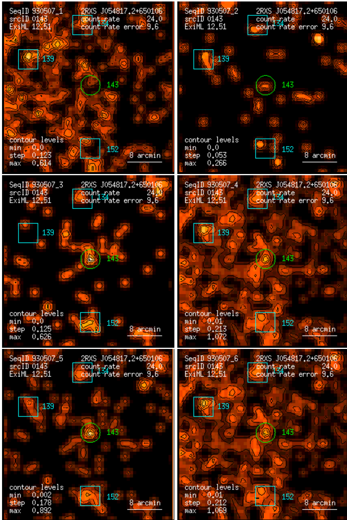
Figure 143: RASS 930507: detection 0143: band rate images, Gaussian filter: (1) PSPC channels 11 – 41, (2) 52 – 90, (3) 91 – 201, (4) 11 – 235, (5) 52 – 201, (6) 11 – 201. Broad band rates in counts/ks. Band rate contour levels in counts/ks/arcmin 2 .
