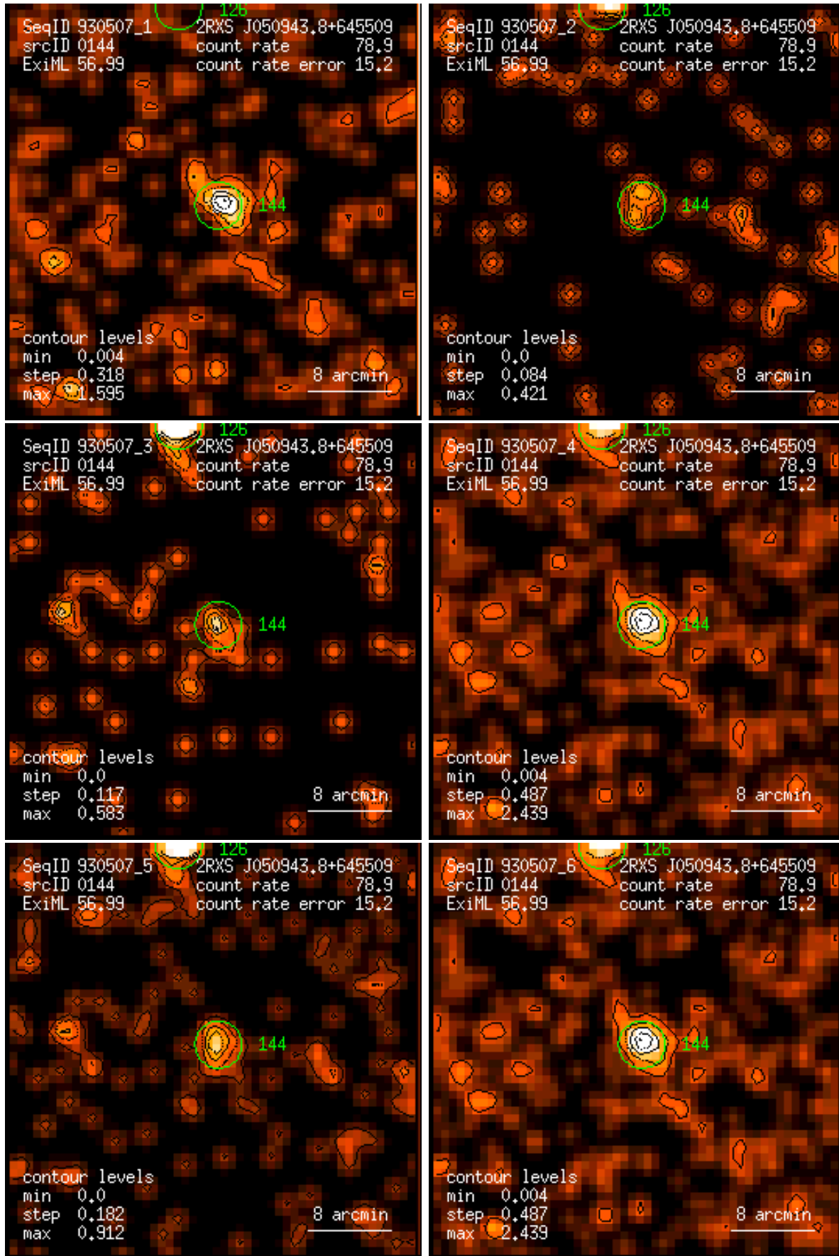
Figure 144: RASS 930507: detection 0144: band rate images, Gaussian filter: (1) PSPC channels 11 – 41, (2) 52 – 90, (3) 91 – 201, (4) 11 – 235, (5) 52 – 201, (6) 11 – 201. Broad band rates in counts/ks. Band rate contour levels in counts/ks/arcmin 2 .
